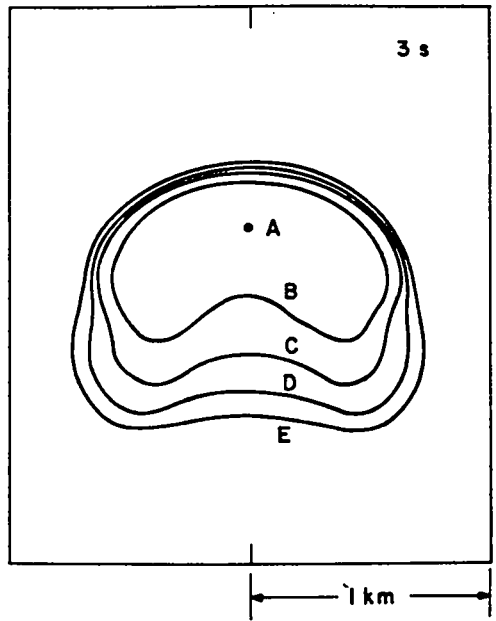
Fig. 15. Isophotes in the red band (5600 to 6800 Å) at selected times. The radiance factor between successive isophotes is 1.38. The brightest points are marked "A."
